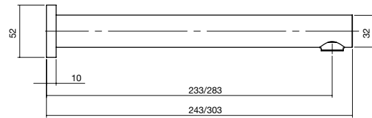
wall outlet
