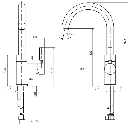
gooseneck sink mixer
