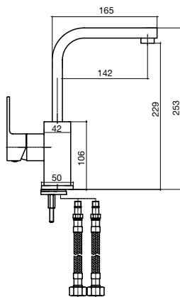
gooseneck sink mixer small
