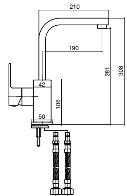
gooseneck sink mixer large
